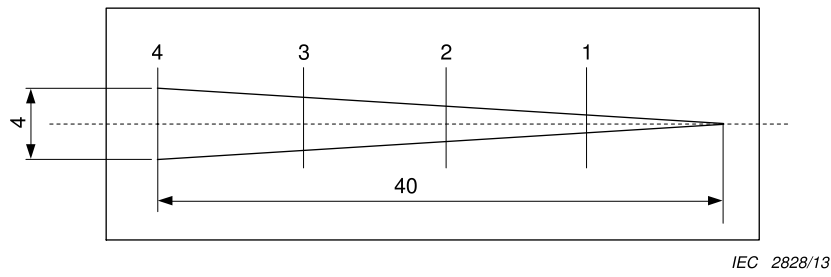
Figure GG.3 – Isosceles triangle arrow test gauge
