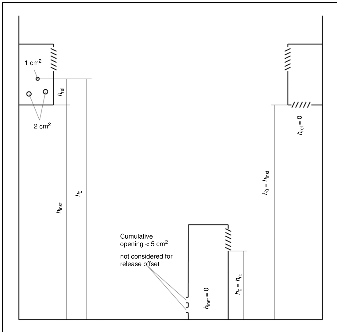
Figure GG.5 – Relevant heights h_{\text{inst}} , h_0 and h_{\text{rel}} for calculation of A_{\text{min}} and m_{\text{max}}
